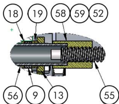
DETAIL D
